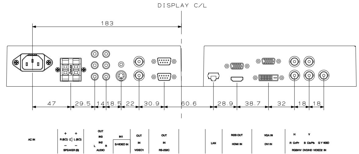
I/O TERMINAL
