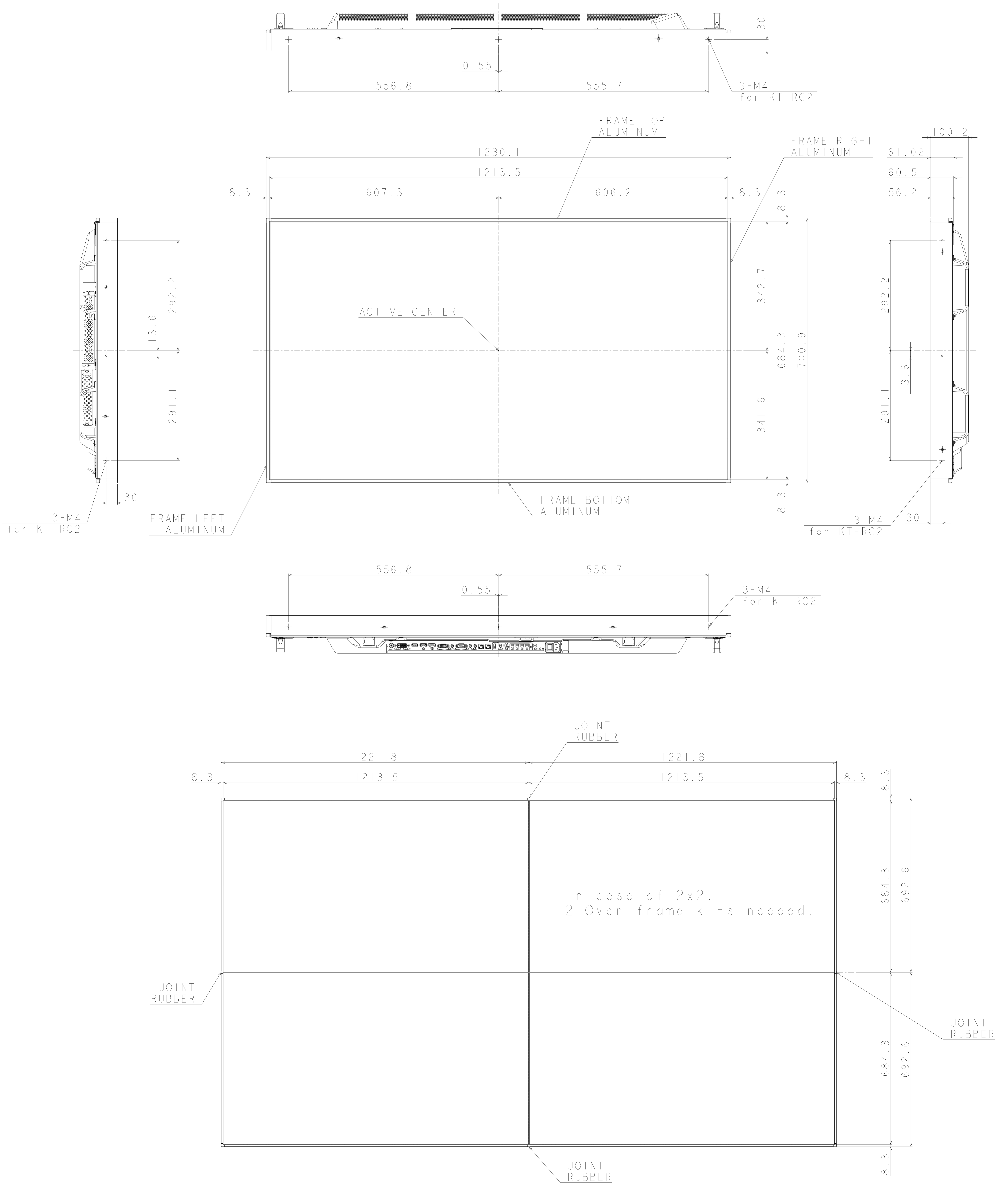
X554UNS with KT-55UN-OF2 OUTLINE DRAWING
